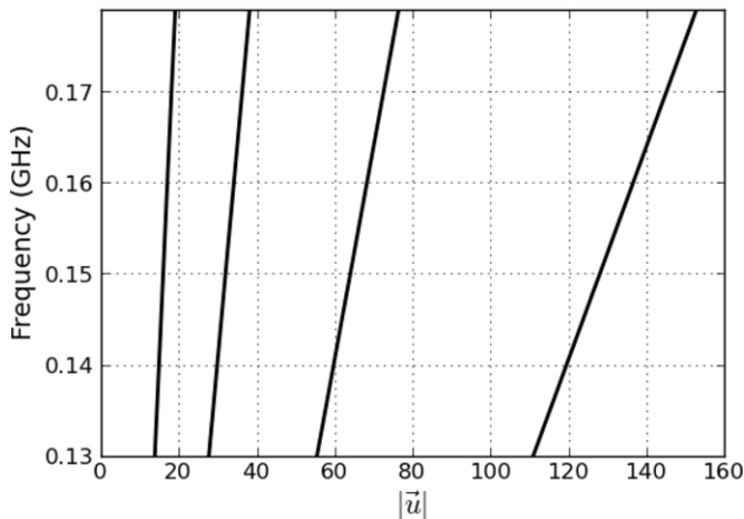
Figure 4. Tracks sampled by baselines measuring 16, 32, 64, and 128 wavelengths (at 150 MHz), as a function of observing frequency, in (u, v) space (solid, bottom axis). The frequency dependence of the wavemode sampled by an interferometer is one of the major complicating factors in foreground removal and is also the reason that emission from celestial sources at different positions on the sky maps to different regions of delay space. The delay transform described in Section 2 extracts Fourier modes measured along these tracks, rather than strictly along the frequency axis.
