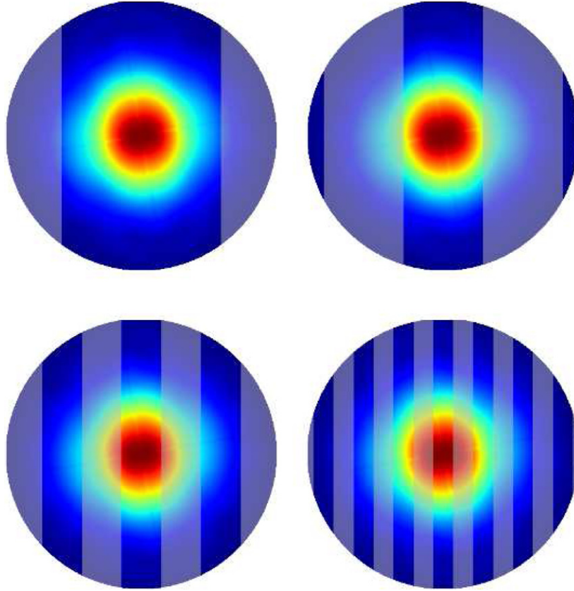
Figure 6. Delay bins (alternating shaded/unshaded regions) resulting from the delay transform applied to an 8 MHz band of data from east–west oriented baselines of length 32 (upper-left), 64 (upper-right), 128 (lower-left), and 256 (lower-right) m, corresponding to 16, 32, 64, and 128 wavelengths, respectively. Bin responses are shown projected over the spatial response of the PAPER primary beam at 150 MHz. Color scale illustrates normalized power response, ranging from 0 (blue) to 1 (red) at zenith. Note that the number of delay bins shown overlapping the field of view in this figure corresponds to the number of shaded bins in Figure 5 that indicate regions where perfectly smooth-spectrum celestial emission can enter a delay mode as a result of instrumental response.
