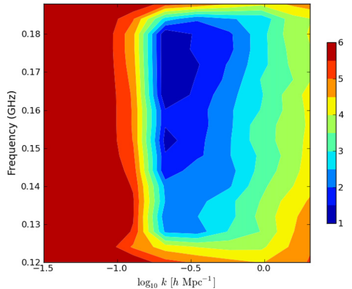
Figure 9. \Delta^2(k) vs. frequency and \log_{10}(k) , computed using the delay transform, for simulated measurements of a 16-wavelength baseline at 150 MHz. Different frequency values denote the centers of the various 8 MHz sub-bands over which the delay transform is applied. As detailed in Section 4, these simulations include the effects of noise, data flagging, and foreground emission consisting of galactic synchrotron emission and extragalactic point sources with power-law spectra. Color denotes \log_{10}(\text{mK}^2) , ranging from 1 (blue) to 6 (red). In this plot, the horizon limit on the geometric delay of celestial emission is clearly seen in the rapid falloff of bright foreground emission vs. k . The subsequent rise in temperature vs. k is the result of k^3 dependence of \Delta^2(k) multiplying flat thermal noise.
