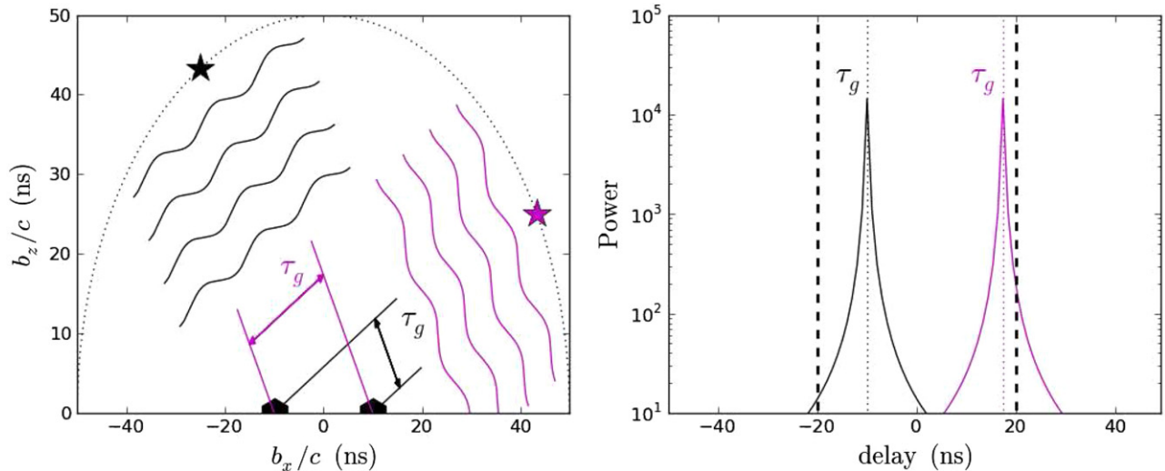
Figure 1. Geometric interpretation of the delay spectrum measured by an interferometer. The left plot shows how two sources with identical spectra can have differing geometric delays ( \tau_g ) owing to their positions relative to the two antennas being correlated. The right plot shows how a strictly geometric interpretation of a delay spectrum is violated by the fact that the Fourier transform of the spectrum of each source also enters the delay spectrum centered at the appropriate \tau_g . This is a manifestation of the convolution expressed in Equation (11). Thick dashed lines denote the maximum possible geometric delays, as imposed by the horizon. While the geometric delay associated with a source cannot exceed the horizon limit, sidelobes associated with the delay transform of the source spectrum do (right plot, magenta).
