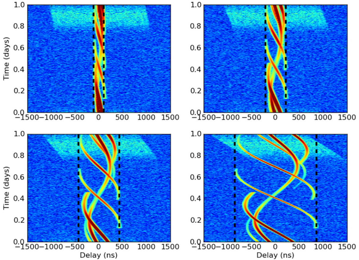
Figure 3. Delay spectra measured by baselines of four different lengths for a simulated sky consisting of several celestial sources, whose spectra are shown in Figure 2. The upper-left, upper-right, lower-left, and lower-right plots show delay spectra obtained by Fourier transforming a 60 MHz band centered at 150 MHz with a Blackman–Harris windowing function (Harris 1978) for east–west baselines of length 32, 64, 128, and 256 m (16, 32, 64, and 128 wavelengths at 150 MHz), respectively. Color scale denotes \log_{10} -Jy amplitude, ranging from 1 (blue) to 5 (red). As in Figure 1, emission from sources with power-law spectra remains confined within the horizon limits (dashed vertical lines), while emission from the source with an unsmooth spectrum (top region of each panel, corresponding to the source plotted in cyan in Figure 2) extends beyond these limits. (A color version of this figure is available in the online journal.)
