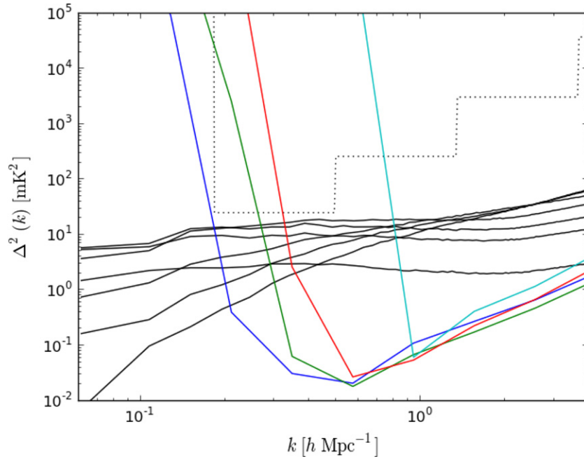
Figure 8. Predicted PAPER 132 power-spectrum sensitivity from P12 (dotted black), re-plotted to show binning intervals in k , and modified to only include contributions at each k -value from baselines that do not show foreground corruption there, is overlaid on noiseless simulations of contamination by smooth-spectrum foreground emission observed by baselines of length 16 (blue), 32 (green), 64 (red), and 128 (cyan) wavelengths at 150 MHz. See Section 4 for simulation details. Simulated 21 cm reionization power spectra from Lidz et al. (2008), with ionization fractions of 0.02, 0.15, 0.21, 0.54, 0.82, 0.96, (black curves, top to bottom, respectively, on plot right) are also shown, projected to redshift 7.9, corresponding to 160 MHz. It should be noted that these predicted power spectra are considerably more pessimistic than those used in Beardsley et al. (2012). Judicious use of windowing functions produces falloff in foreground emission at a characteristic scale that depends on baseline length. The rise of foreground emission at higher k is not noise, but rather is the result of sidelobes of smooth-spectrum foreground emission that are not fully suppressed by the windowing and deconvolution steps used to compute the delay spectrum, multiplied by the k^3 factor in \Delta^2(k) .
