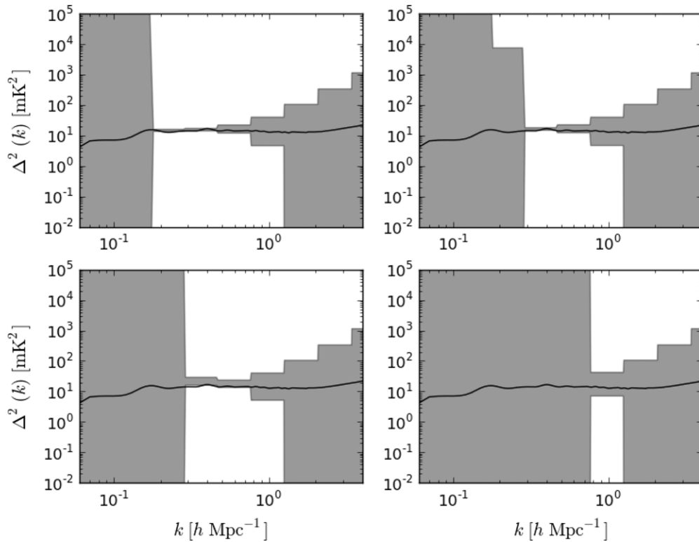
Figure 11. Measured \Delta^2(k) vs. k with shaded 2\sigma error bars for baselines of length 32 (upper-left), 64 (upper-right), 128 (lower-left), and 256 (lower-right) m, corresponding to 16, 32, 64, and 128 wavelengths, respectively, as measured using the delay-spectrum technique. Error bars include contributions from foregrounds and from thermal noise, assuming observations with a future array 100 times more sensitive than a 132-antenna PAPER array observing for 200 days. The dark solid line denotes the true \Delta^2_{21}(k) power spectrum used in the simulation.
