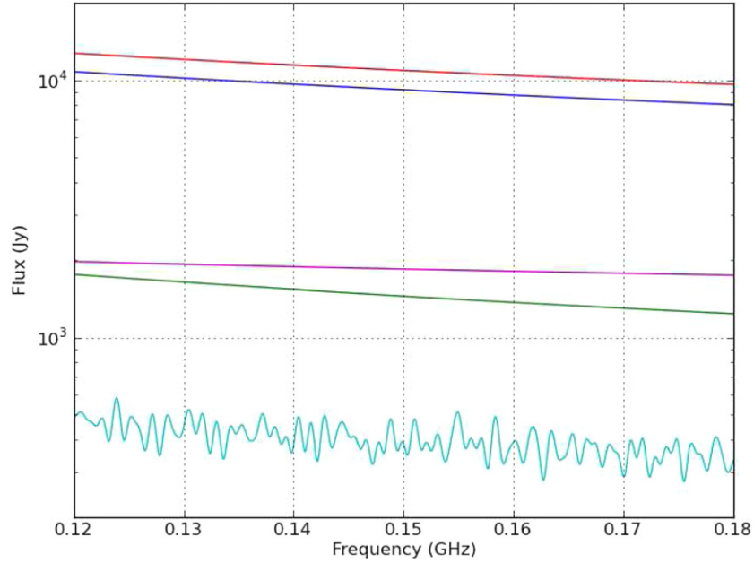
Figure 2. Spectra of five sources at random positions on the sky that were used to generate simulated visibilities from which the delay spectra in Figure 3 were calculated, using a model of PAPER’s primary-beam response. All but one of the sources (cyan) have power-law spectra vs. frequency. (A color version of this figure is available in the online journal.)
