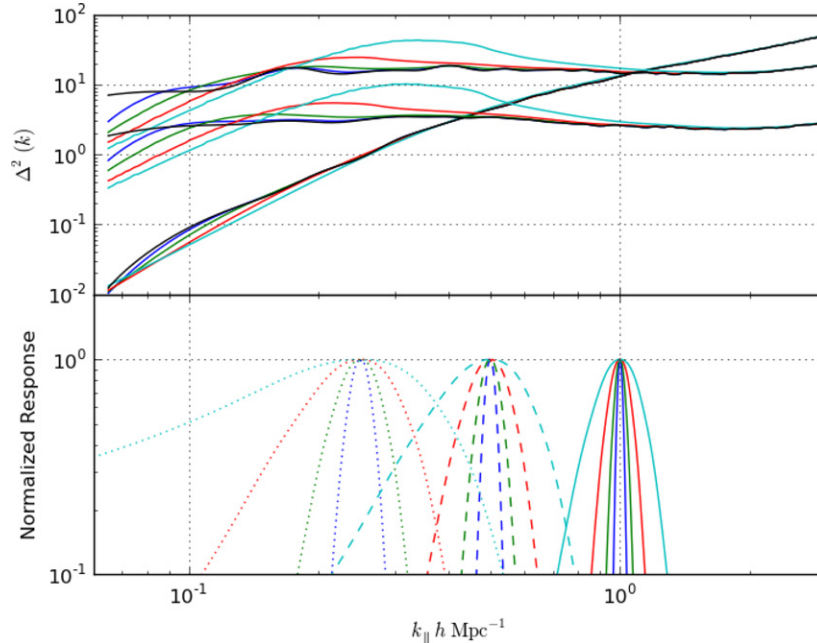
Figure 7. Top: the effect of the delay-transform PSF on measured power spectra of 21 cm reionization, using model power spectra at various stages of reionization from Lidz et al. (2008). Bottom: the k_{||} response ( W_{\tau,b}(\eta) ), from Equation (9) of a delay-transform bin arising from the sloped response in k_{||} shown in Figure 5, integrated over the primary-beam response of a PAPER dipole, at bins centered at k_{||} = 0.25, 0.5 , and 1.0 h \text{ Mpc}^{-1} (dotted, dashed, and solid plots, respectively). Color indicates baseline length in wavelengths at 150 MHz of 16 (blue), 32 (green), 64 (red), and 128 (cyan). The width of the response of a delay-transform bin arises from the inherent scaling of uv -coverage with frequency, or equivalently, from the width of the primary beam in delay space. Only for the longest baselines does mode-mixing substantially affect measurements of the power spectrum of high-redshift 21 cm emission.
