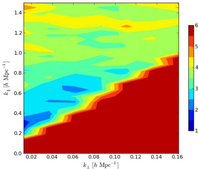
Figure 10. \Delta^2(k) vs. k_\perp and k_\parallel , derived from the same simulations as in Figure 9, but using a single delay-transform band centered at 150 MHz. Color denotes \log_{10}(\text{mK}^2) , ranging from 1 (blue) to 6 (red). In this plot, the broadening of foreground contamination at lower k_\parallel increases as a function of k_\perp , reflecting how the horizon limit in delay space increases as a function of baseline length. The “wedge” of foreground contamination illustrated here parallels the simulated foreground contamination found in Datta et al. (2010) and Morales et al. (2012), and is indicative of the fundamental shape of smooth-spectrum foreground emission as observed by an interferometer that has a frequency-dependent sampling of the uv -plane.
