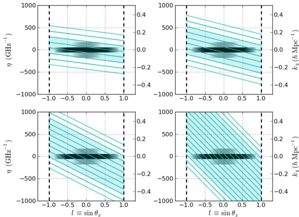
Figure 5. Response in (l, \eta) -coordinates of delay bins measured by baselines of four different lengths, all chosen, without loss of generality, to be in the east–west direction. The gray-scale shading in the center of each plot shows the response of the PAPER primary beam, integrated over the direction perpendicular to the baseline (i.e., in the m -direction, along the delay bins indicated in Figure 6), and Fourier transformed in frequency over an 8 MHz band (centered at 150 MHz) at each l -coordinate to yield \int \tilde{A}(l, m, \eta) dm . Gray scale indicates response relative to peak amplitude in \log_{10} \text{mK}^2 units, ranging from 0 (black) to -2 (white). In this space, the beam spans a broad range of l (it has a wide FWHM) but is fairly narrow in \eta (it is very smooth in frequency). Overlaid on the beam representation are the regions of sensitivity of delay-spectrum bins for baselines of length 32 (upper-left), 64 (upper-right), 128 (lower-left), and 256 (lower-right) m, corresponding to 16, 32, 64, and 128 wavelengths, respectively. The area between two colored lines corresponds to the region to which a single \tau -mode of that baseline’s delay spectrum is sensitive. As in Figure 1, the thick dashed line denotes the horizon cutoff. Each \tau -mode probes a range of \eta -values across the field of view, although shorter baseline lengths reduce the degree to which delay bins mix \eta -modes. To aid the eye, we have shaded \tau -bins that intersect the primary-beam response at greater than 1% of peak amplitude, indicating delay modes where instrumental response scatters perfectly smooth-spectrum celestial emission. For each baseline length, there also exist unshaded delay bins where significant power can only exist if celestial emission itself has structure at sufficiently high \eta (i.e., it has rapidly fluctuating frequency structure). Since foreground emission at these frequencies is predominantly smooth-spectrum (Furlanetto et al. 2006), this approach allows the dominant foregrounds to the 21 cm EoR signal to be avoided by employing antennas with smooth primary beams vs. frequency (to constrain the gray-scale width in the \hat{\eta} -direction) and by employing shorter baselines that minimize the mixing of \eta -modes within delay bins (by flattening the slope of the colored lines).
